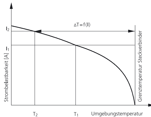
Abb 1. Derating-Kurve
