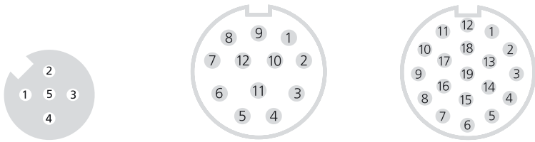
M12x1, Kupplung
